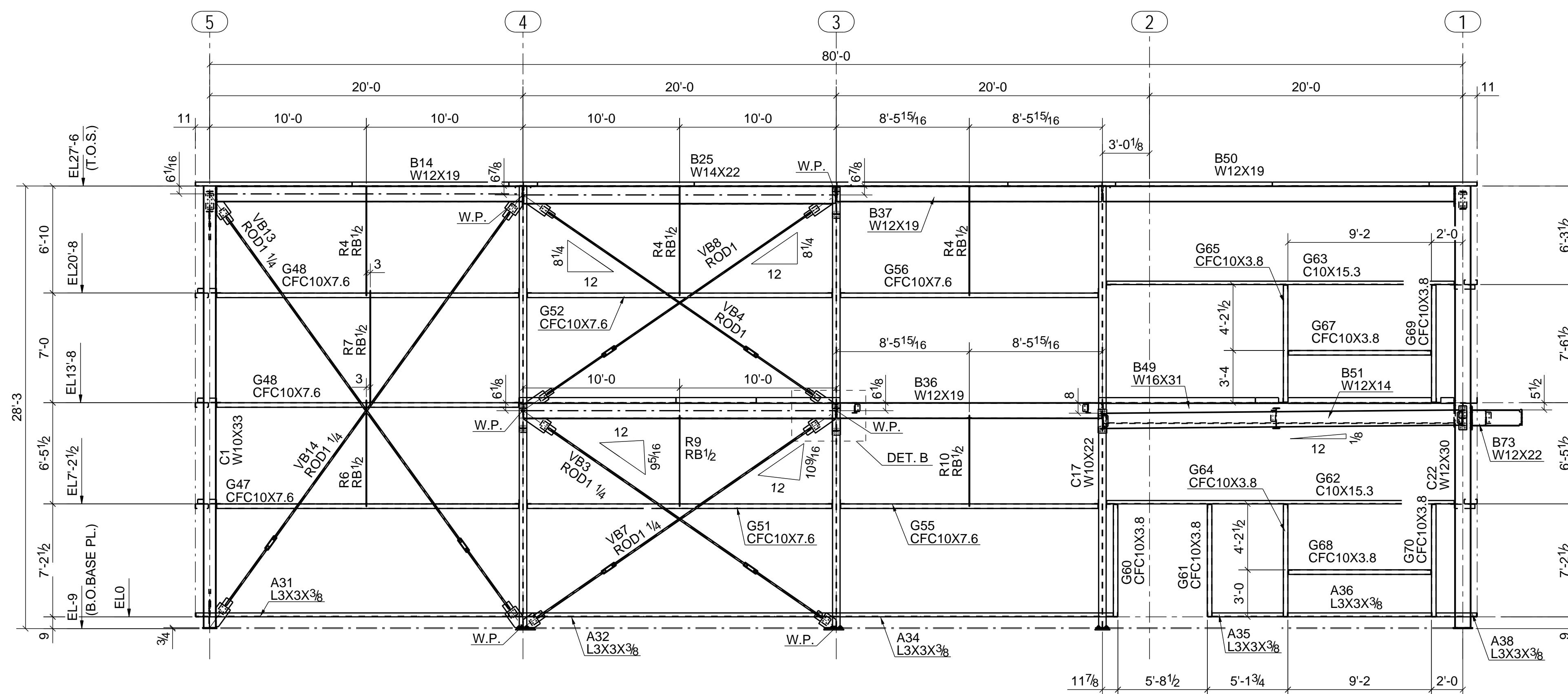
ELEVATION ALONG GRID LINE-G
