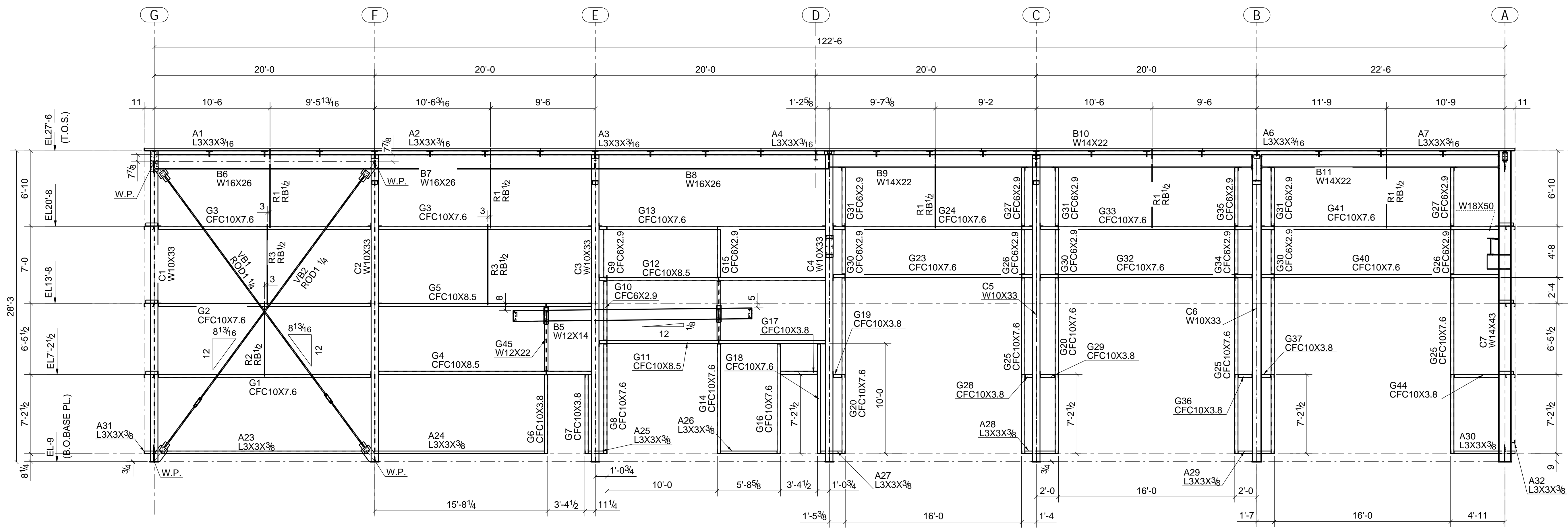
ELEVATION ALONG GRID LINE-5
