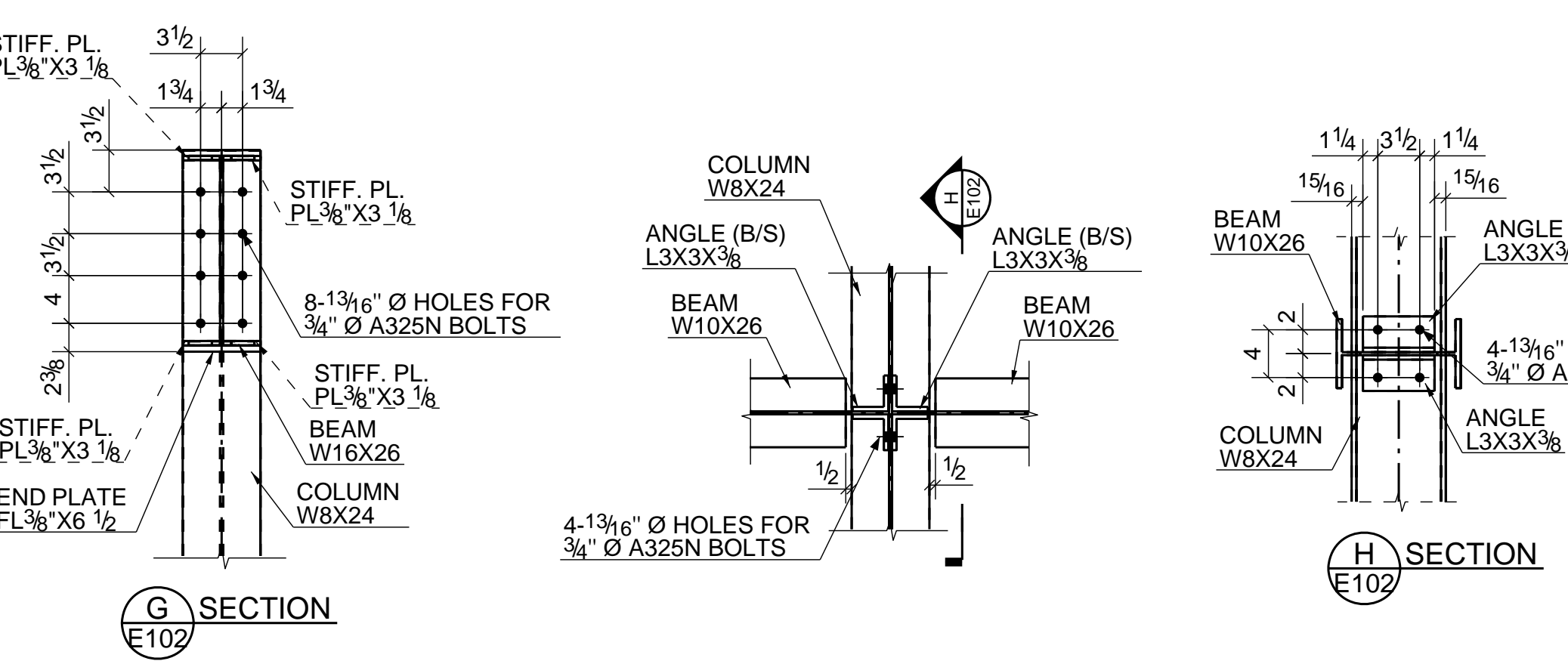
TYPICAL COLUMN TO BEAM CONNECTION DETAILS
