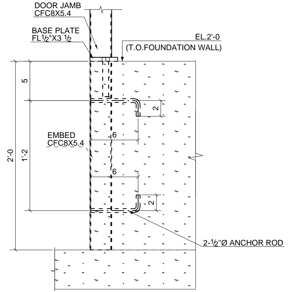
TYPICAL EMBED DETAIL
