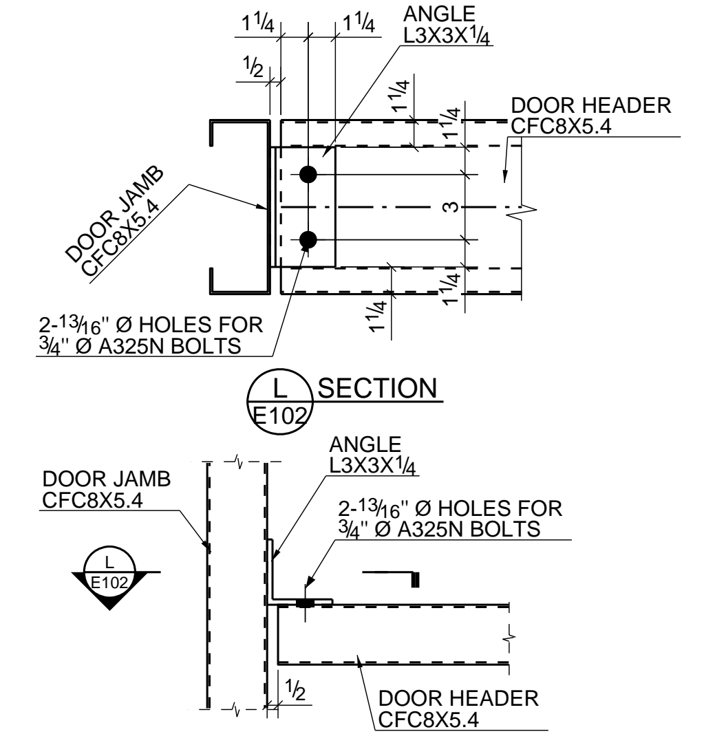
TYPICAL DOOR HEADER CONNECTION DETAIL
