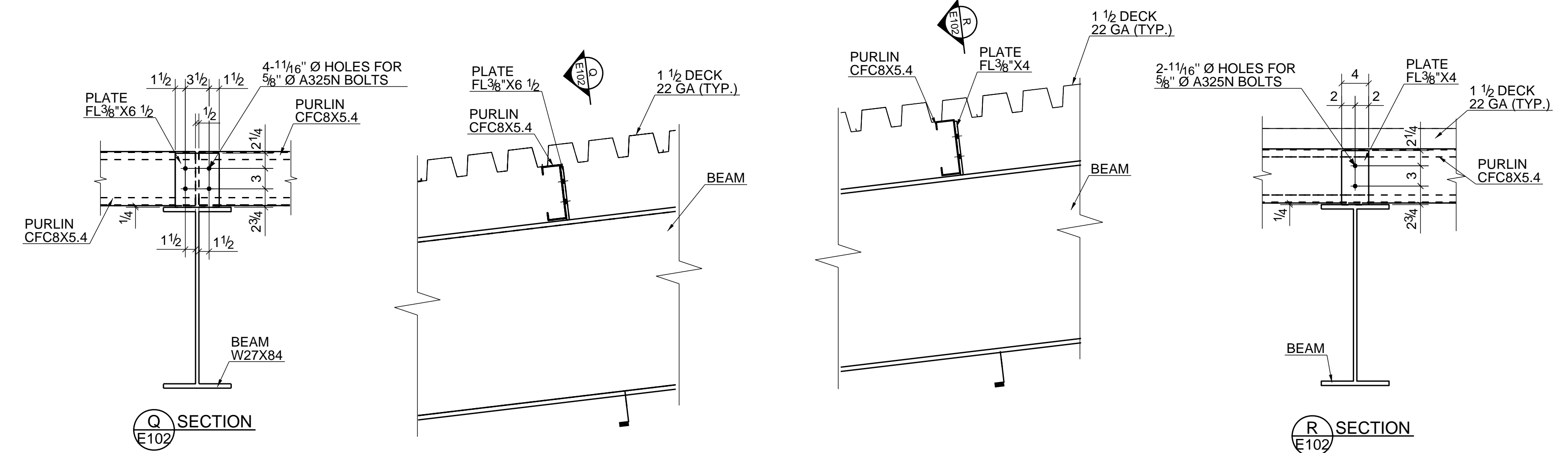
TYPICAL PURLIN CONNECTION DETAILS
