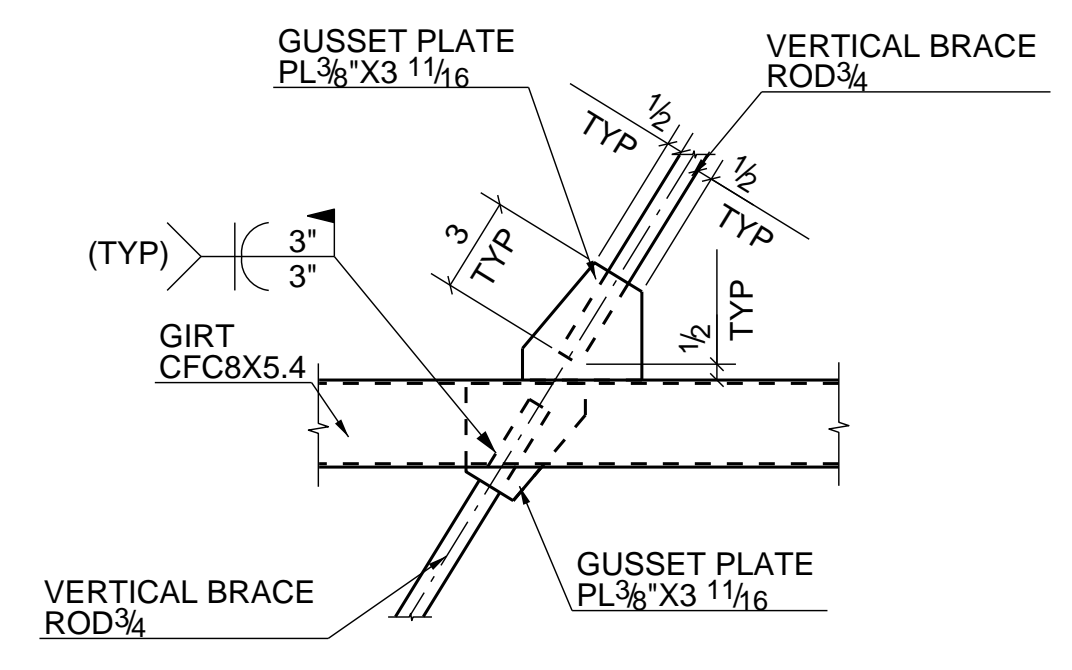
TYPICAL BRACE CONNECTION DETAIL
