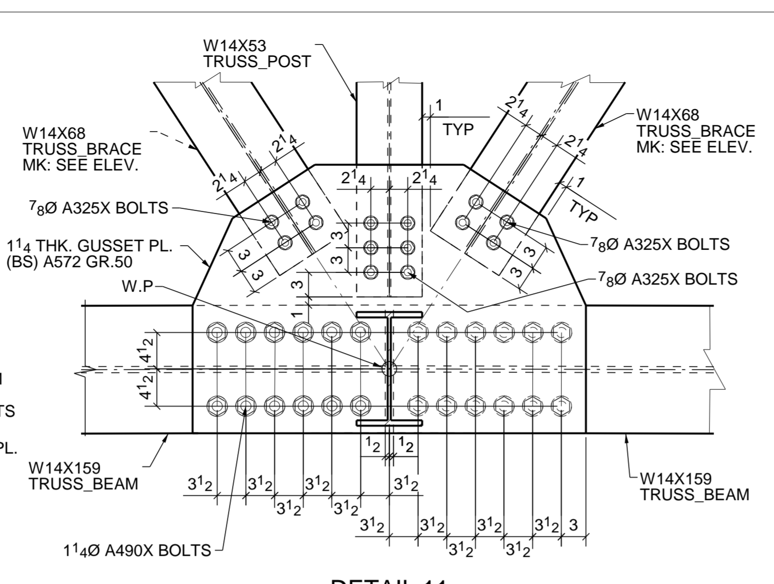
DETAIL 11 (REF: 19/S503)
