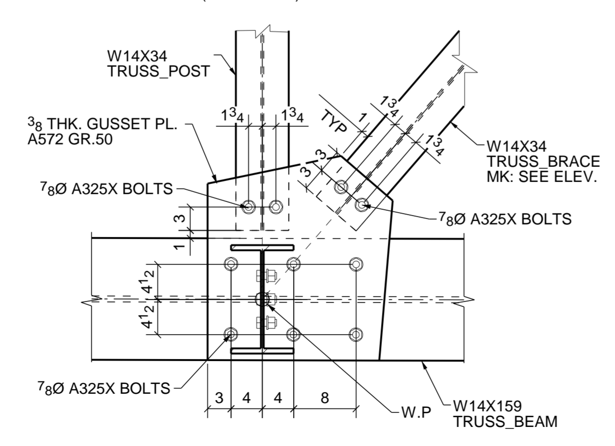
DETAIL 19 (REF: 3/S503)
