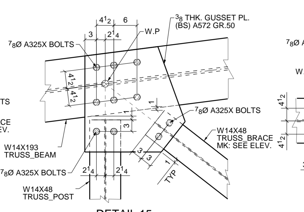
DETAIL 15 (REF: 3/S503)
